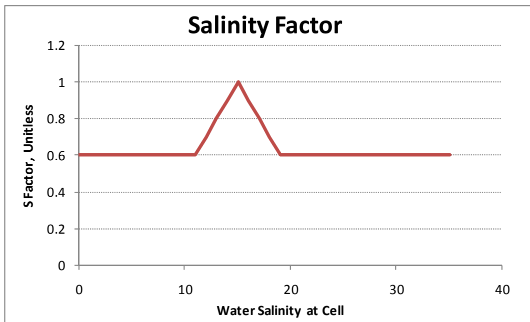
Graph showing predicted salinity correction factors (S) with the following parameters: \text{Salinity}_{\text{TMax}} = 15 ; \text{TMaxZone} = 10 ; \text{S}_{\text{NonTMax}} = 0.6
