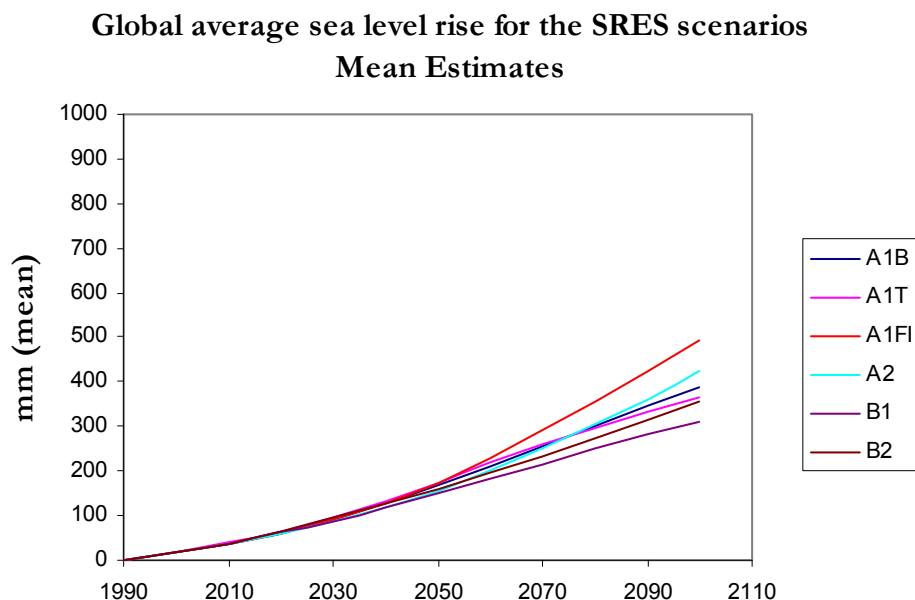
Figure 2: Summary of SRES Scenarios
