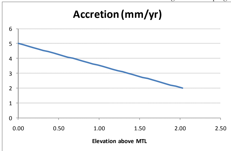
Graph showing predicted accretion rates as a function of elevation with the following parameters: Min. Accretion = 2 mm/year; Max Accretion = 5 mm/year; Min Elev. = 0 m; Max Elev. = 2.02 m; a=-0; b=0. c=1.
