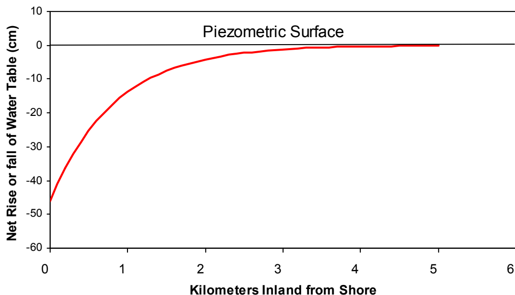
Figure 5: Water Table Rise Near Shore, Based on Carter et al., 1973
