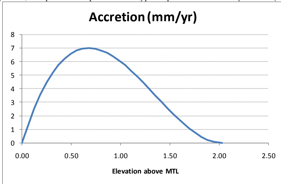
Graph showing predicted accretion rates as a function of elevation with the following parameters: Min. Accretion = 0 mm/year; Max Accretion = 7 mm/year; Min Elev = 0 m; Max Elev = 2.02 m; a=-1; b=1. c=0.
