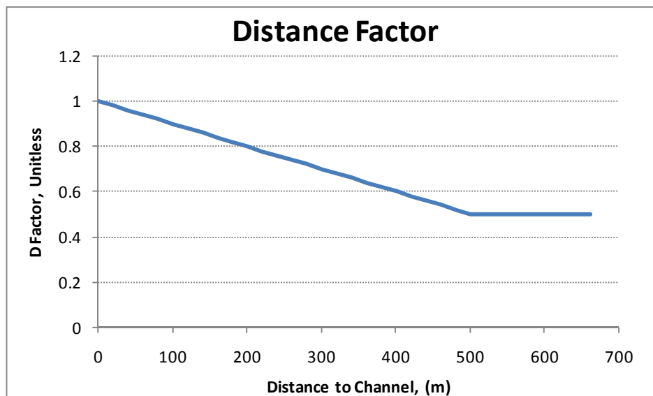
Graph showing predicted distance correction factors with the following parameters: D_{min} = 0.5 ; DistEffect = 500 meters.
